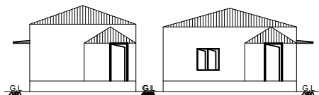
FRONT ELEVATION
