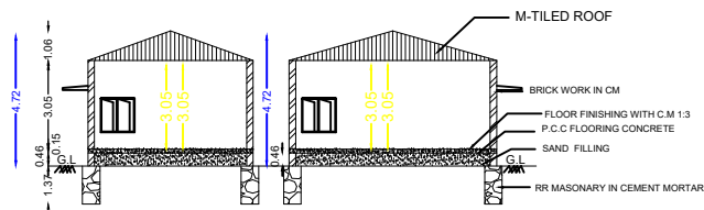
SECTION A - B
