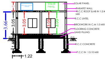
SECTION ON "MG"
