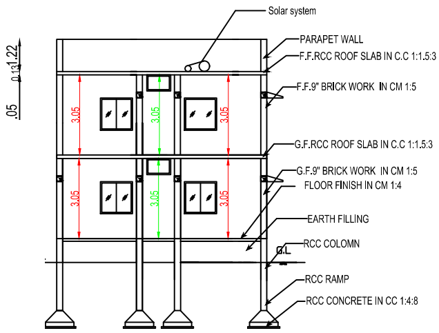
SECTION ON AA & BB
