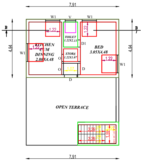
FIRST FLOOR PLAN PROPOSED BUILDING (SCALE 1:100)
