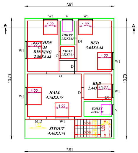
GROUND FLOOR PLAN PROPOSED BUILDING (SCALE 1:100)
