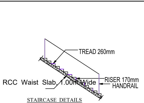
STAIRCASE DETAILS
