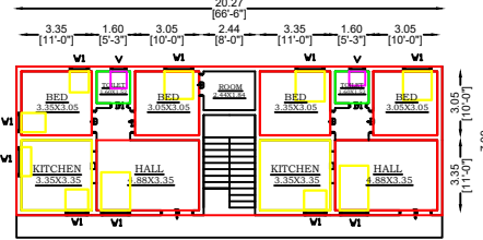
FIRST FLOOR PLAN [PROPOSED-EAST]
