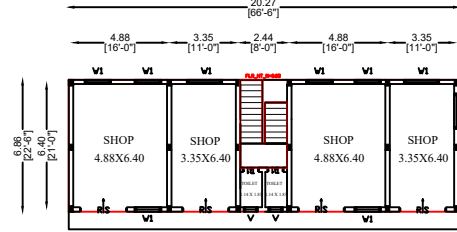
GROUND FLOOR PLAN [EXISTING-WEST]
