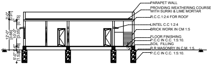
SECTION - "A-B"
