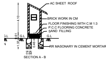
SECTION A - B
