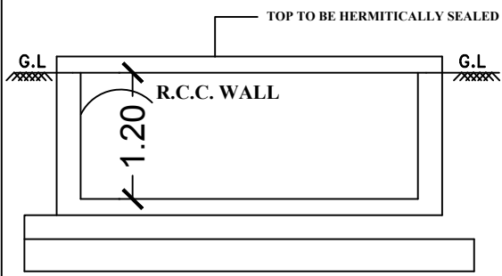
RWH_CAPACITY_L=2160LTRS
