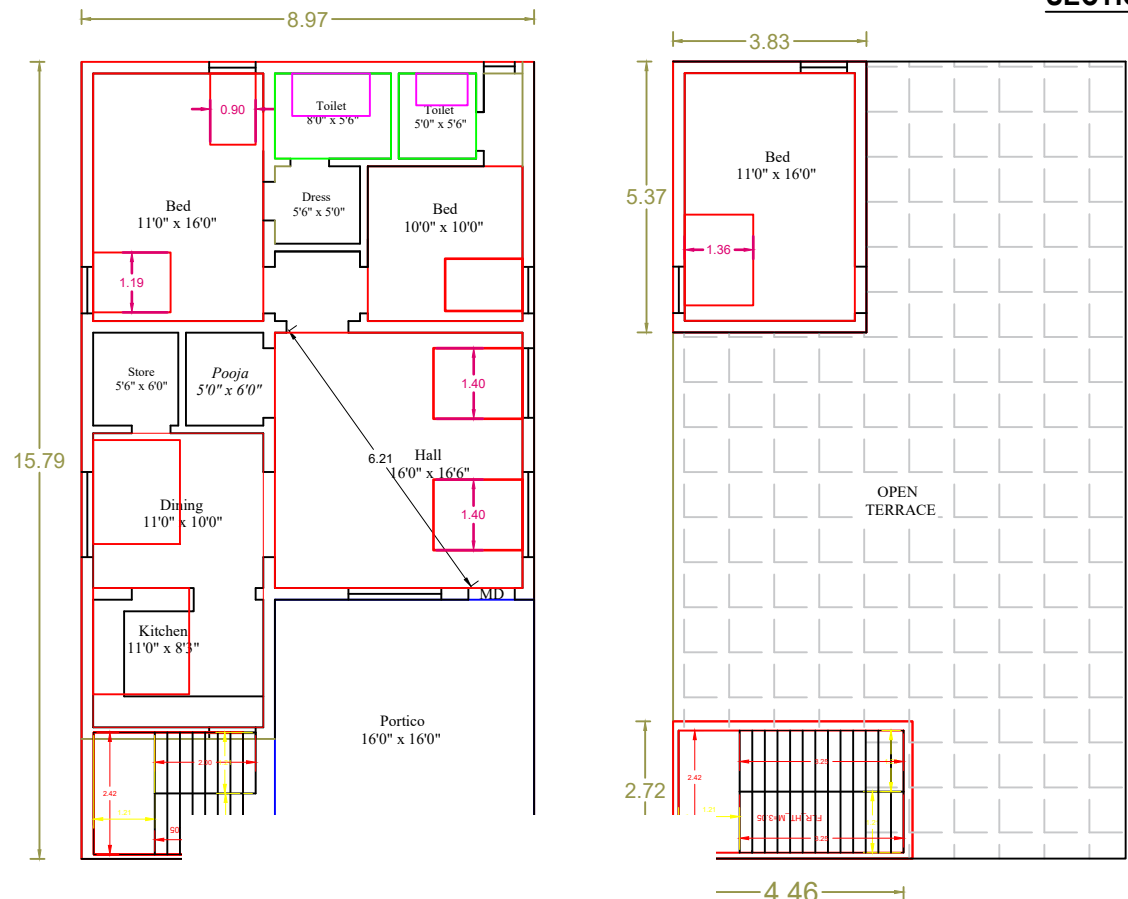
PRO.FIRST FLOOR PLAN.
