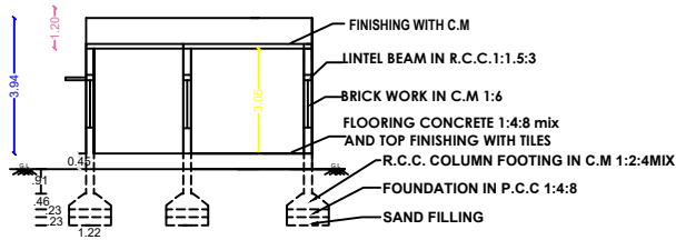
SECTION-AB
