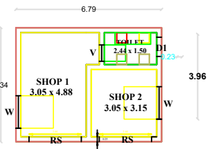
PRO. GROUND FLOOR PLAN
