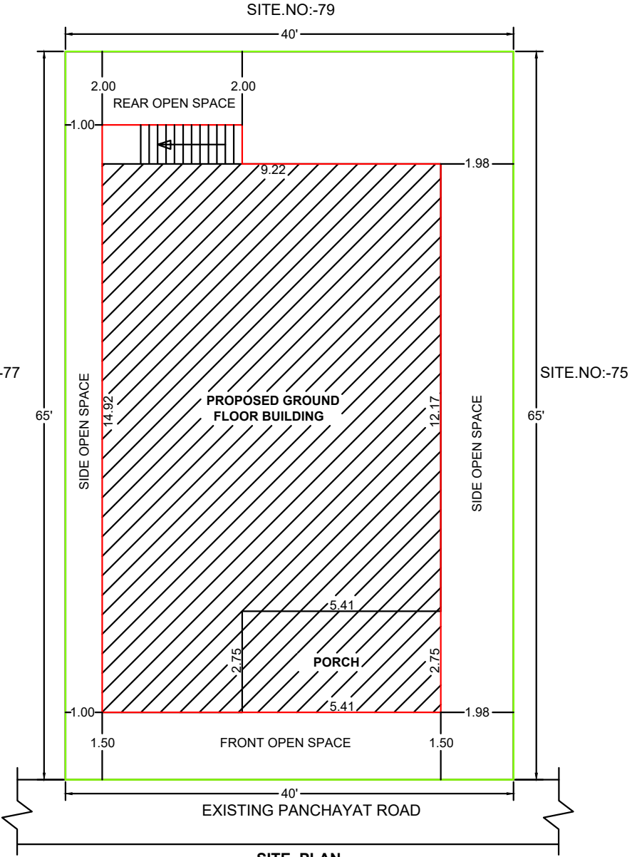
SITE PLAN SCALE 1 CM = 1 M
