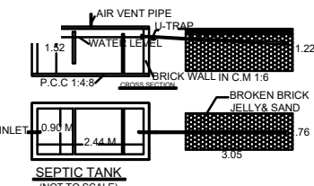
SEPTIC TANK (NOT TO SCALE)
