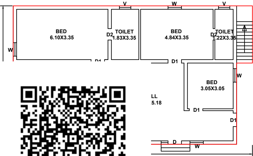
FLOOR PLAN SCALE 1 CM = 1 M
