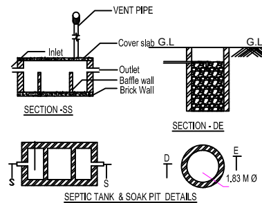
SEPTIC TANK & SOAK PIT DETAILS
