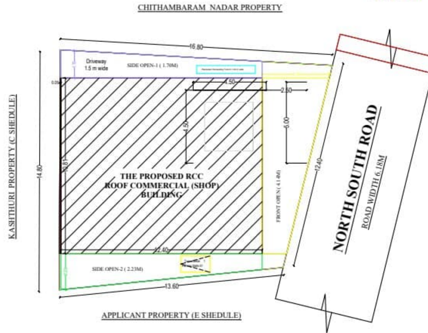
SITE PLAN
