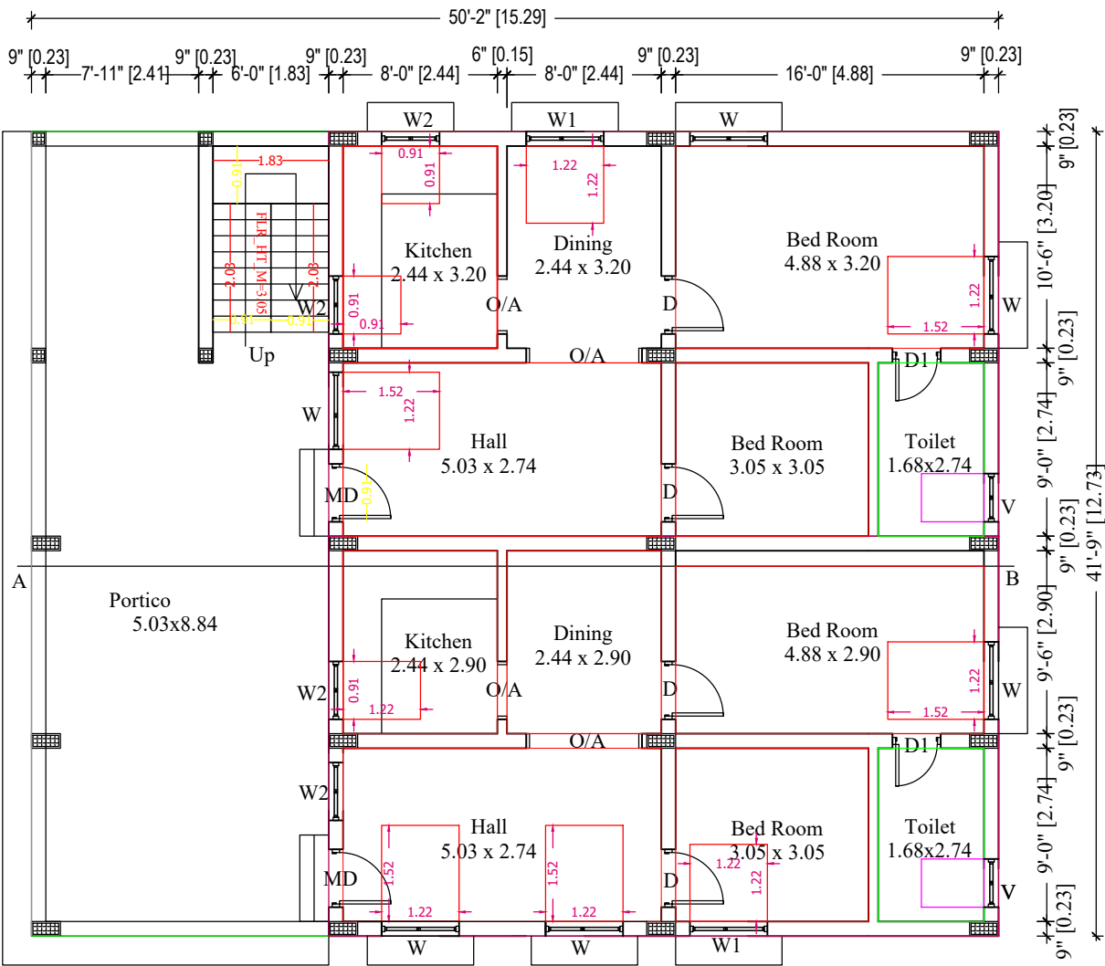
EXI. GROUND FLOOR PLAN
