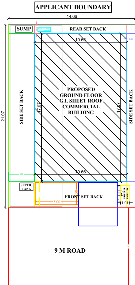
SITE PLAN
