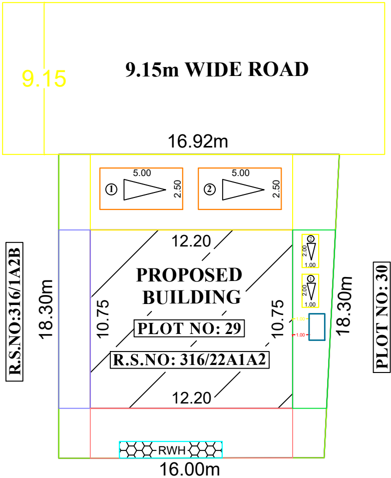
PLOT NO: 28 SITE PLAN SCALE-1:500
