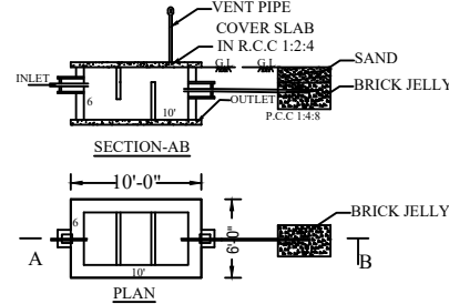
SEPTIC TANK & DISPERSION TRENCH DETAILS SCALE- 1:100
