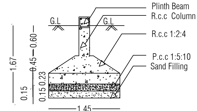
COLUMN FOOTING DETAILS
