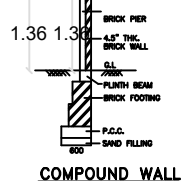
COMPOUND WALL
