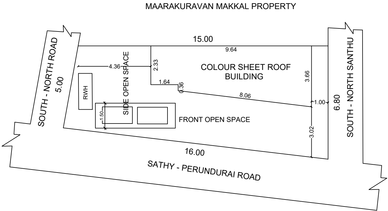
SITE PLAN
