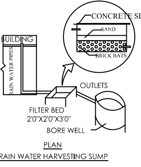
RAIN WATER HARVESTING SUMP
