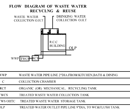
FLOW DIAGRAM OF WASTE WATER RECYCLING & REUSE
