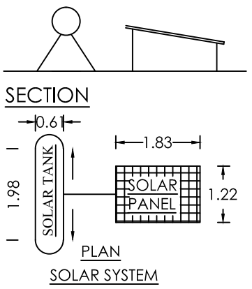
SOLAR SYSTEM
