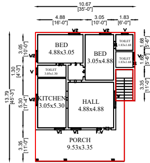
GROUND FLOOR PLAN [EXISTING-EAST]
