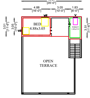
FIRST FLOOR PLAN [PROPOSED-EAST]
