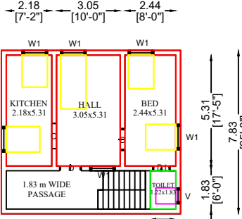
SECOND FLOOR PLAN [PROPOSED-EAST]
