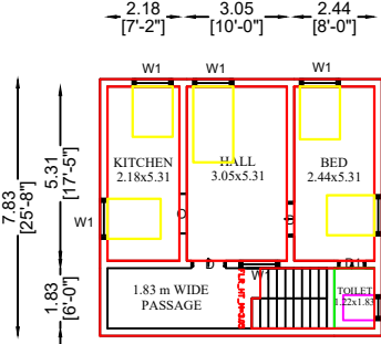
FIRST FLOOR PLAN [PROPOSED-EAST]
