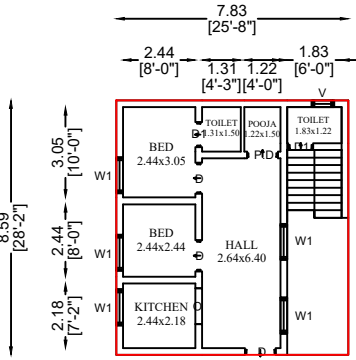
GROUND FLOOR PLAN [EXISTING-EAST]
