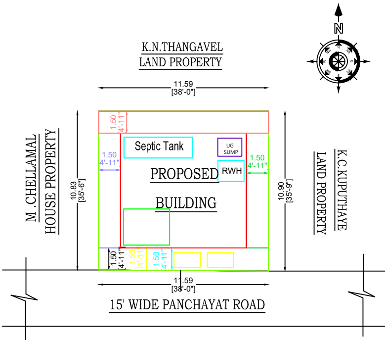
SITE PLAN
