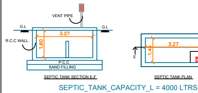
UG SUMP DETAILS
