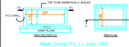
SEPTIC TANK DETAILS
