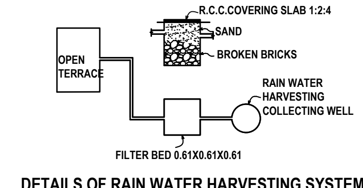
DETAILS OF RAIN WATER HARVESTING SYSTEM
