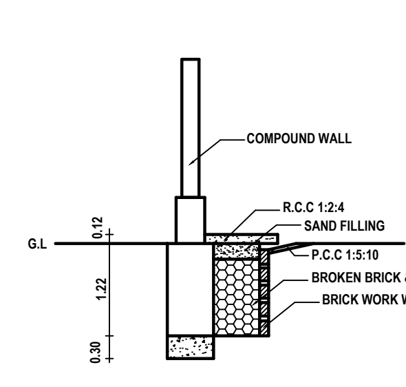
PLINTH BOUNDARY PERCOLATION PIT
