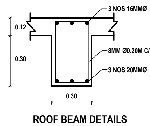
ROOF BEAM DETAILS
