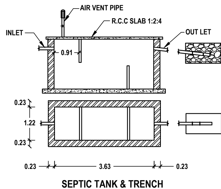
SEPTIC TANK & TRENCH
