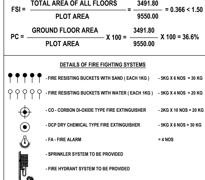
DETAILS OF FIRE FIGHTING SYSTEMS
