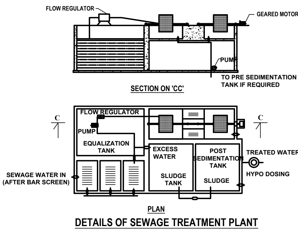
DETAILS OF SEWAGE TREATMENT PLANT
