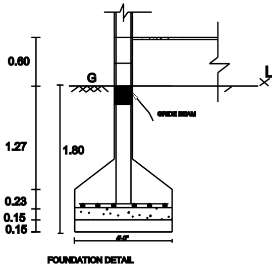
FOUNDATION DETAIL
