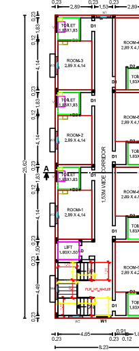
THIRD FLOOR PLAN
