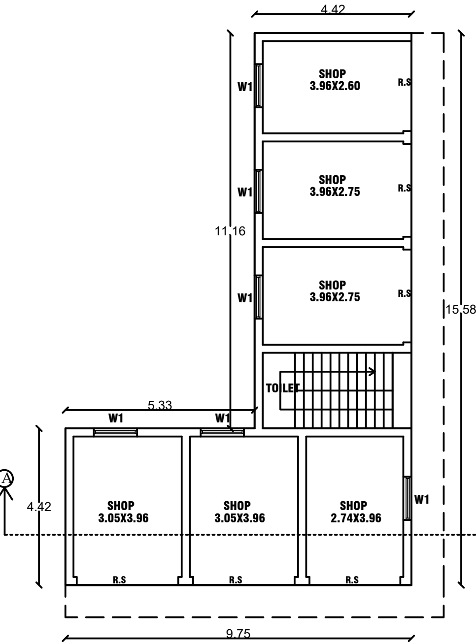
GROUND FLOOR PLAN SOUTH FACING PLAN
