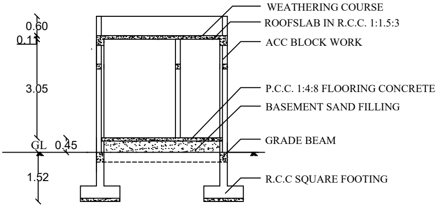
CROSS SECTION ON 'AA'
