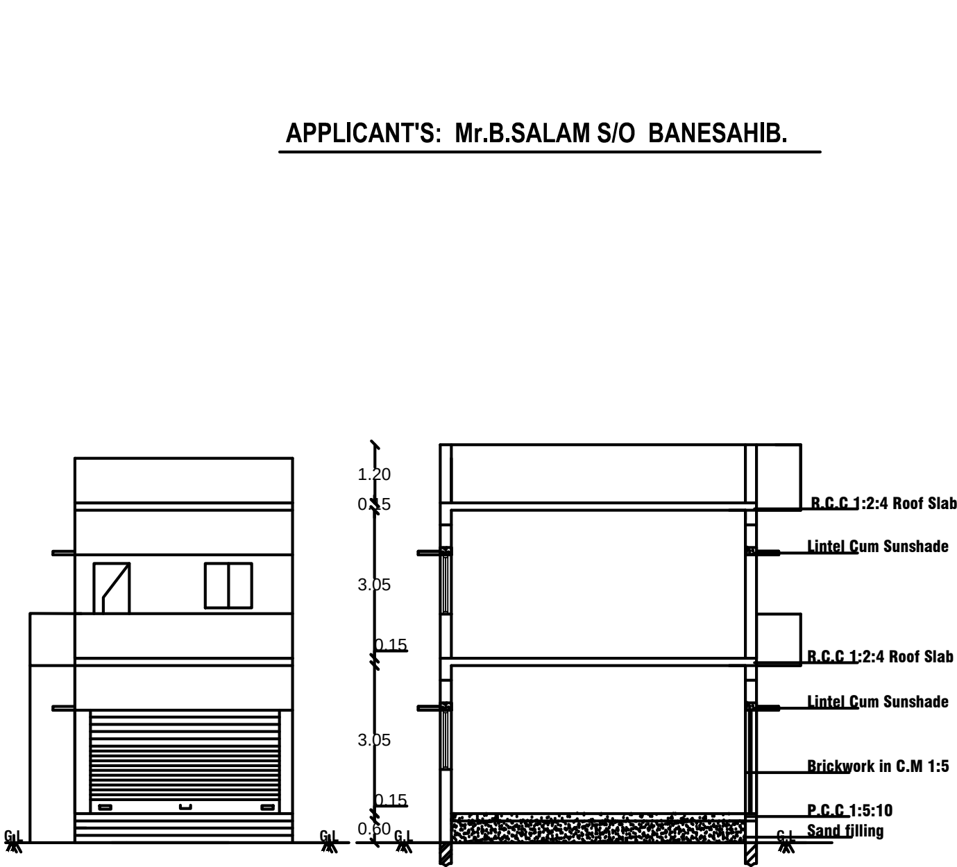
FRONT ELEVATION
