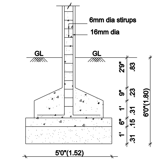
COLUMN FOUNDATION DETAIL SCALE (1:50)
