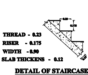
DETAIL OF STAIRCASE
