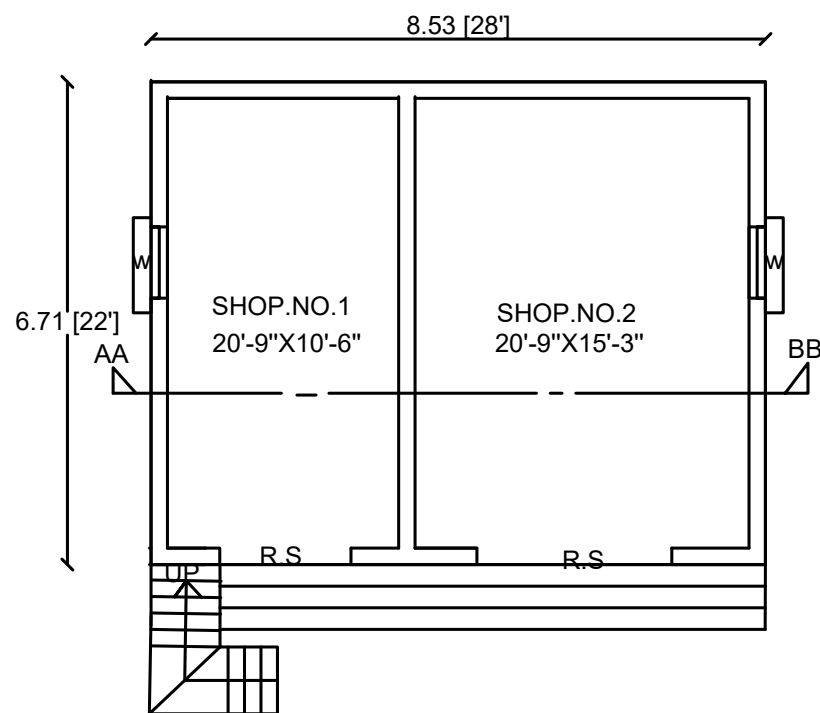
GROUND FLOOR PLAN EAST FACING PLAN
