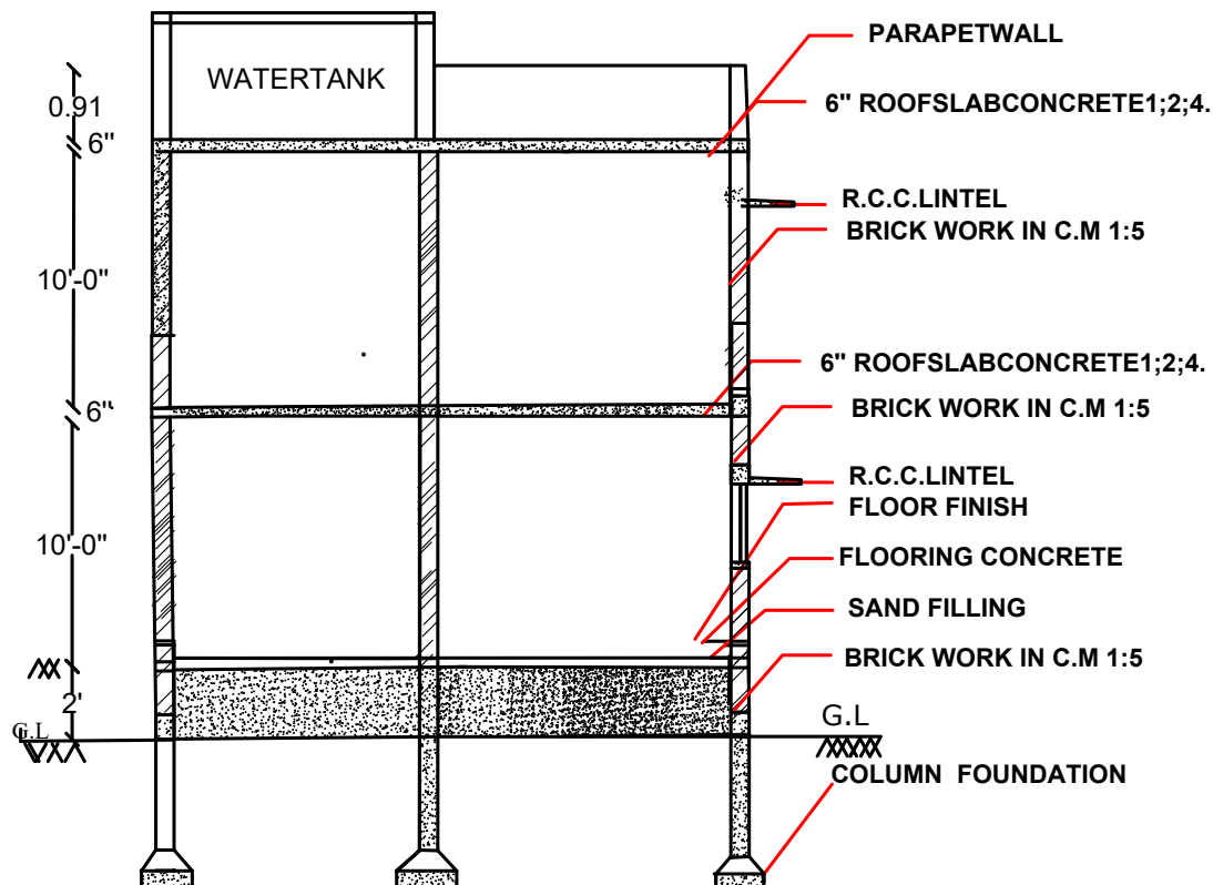
SECTION ON AA & BB
