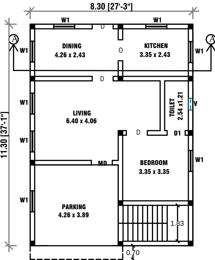
GROUND FLOOR PLAN WEST FACING PLAN
