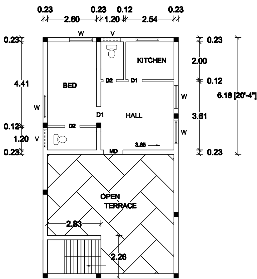
FLOOR01
