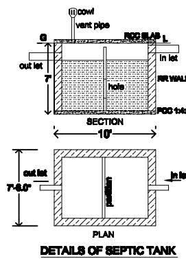
DETAILS OF SEPTIC TANK
