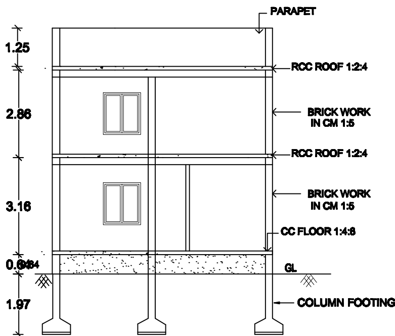
SECTION AB
