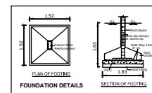
FIGURE 1. FOUNDATION DETAILS
