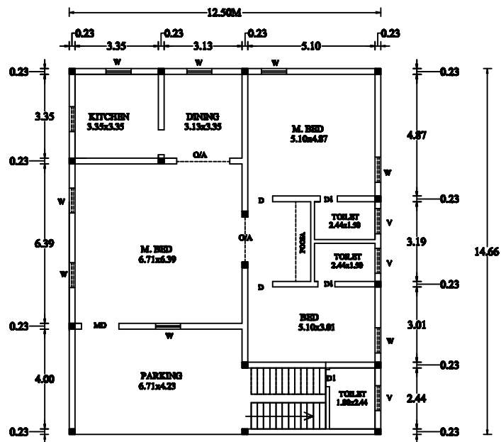
FLOOR GROUND
