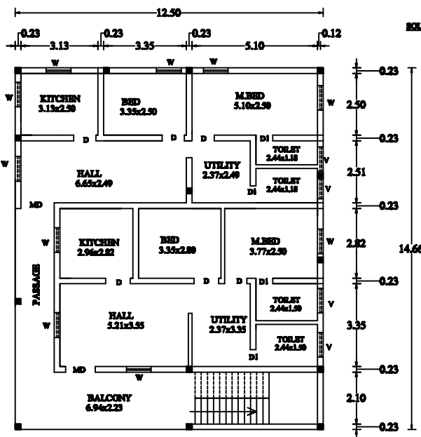
FLOOR 01
