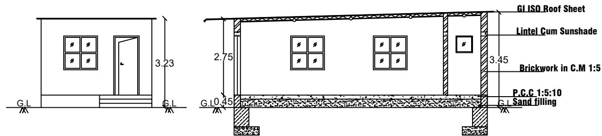
FRONT ELEVATION
