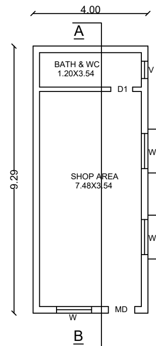
PROPOSED GROUND FLOOR
