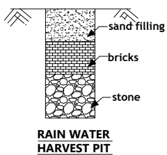
RAIN WATER HARVEST PIT
