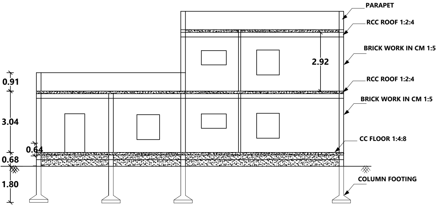
SECTION AB
