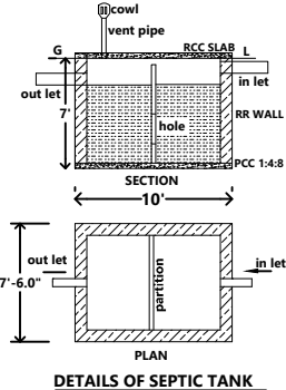
DETAILS OF SEPTIC TANK
