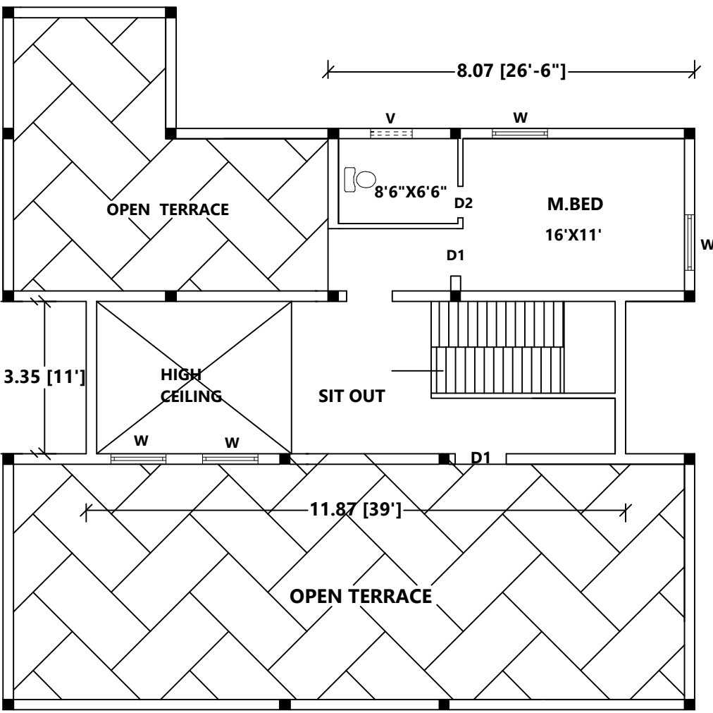
FLOOR01
