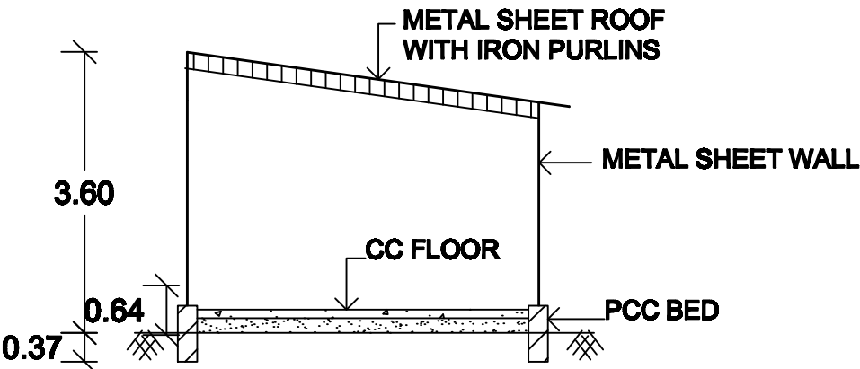
SECTION AB
