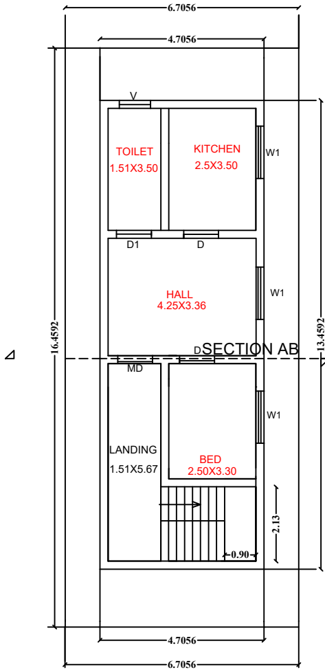
FLOOR01
