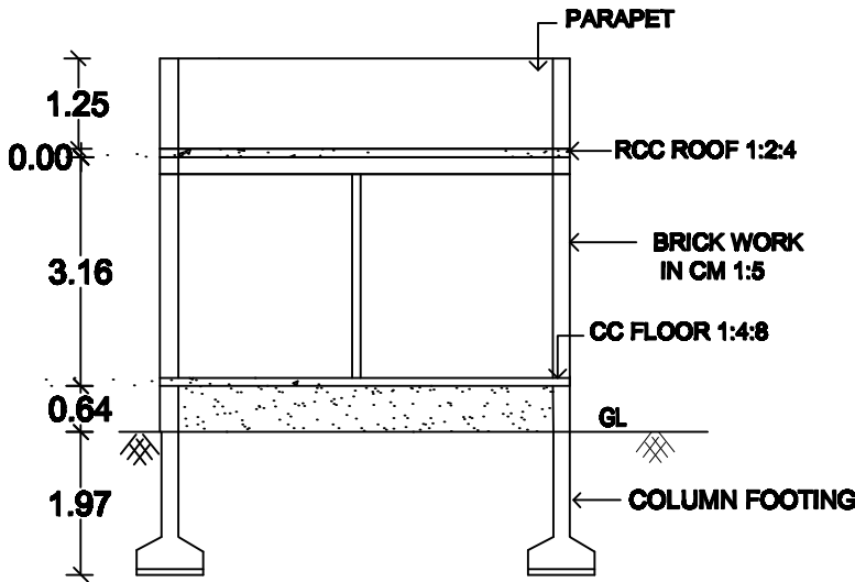
SECTION AB
