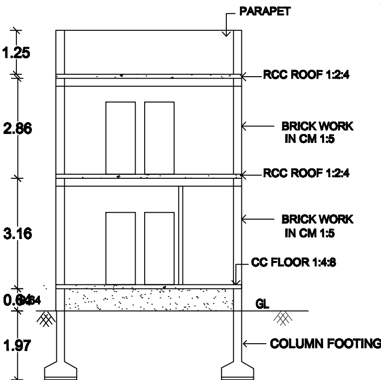
SECTION AB
