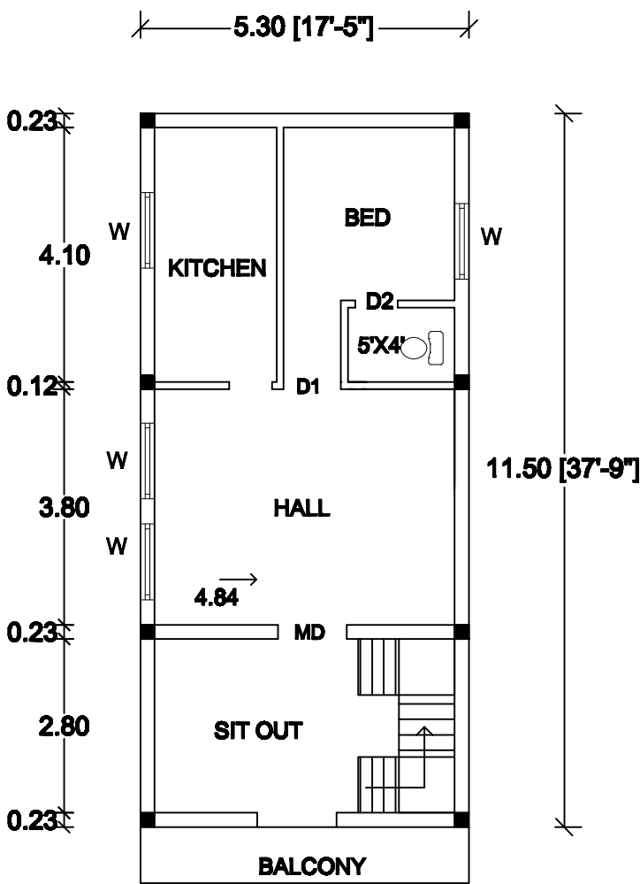
FLOOR01
