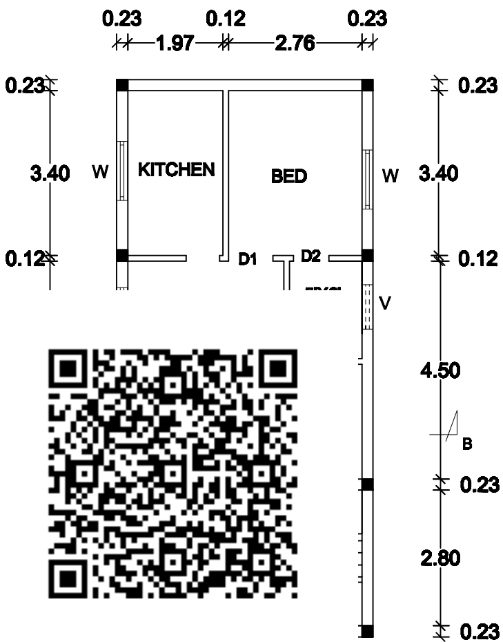
FLOOR GROUND
