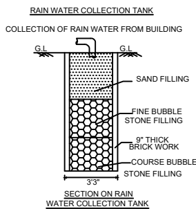
SECTION ON RAIN WATER COLLECTION TANK
