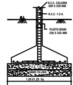
FOUNDATION DETAILS
