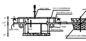
SEPTIC TANK DETAILS
