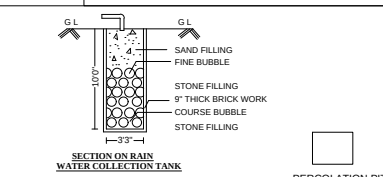
SECTION ON RAIN WATER COLLECTION TANK
