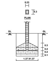
COLUMN DETAILS (NOT TO SCALE)
