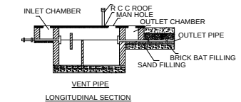
TYPICAL DETAILS OF SEPTITANK
