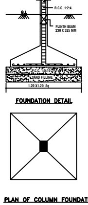
PLAN OF COLUMN FOUNDATION
