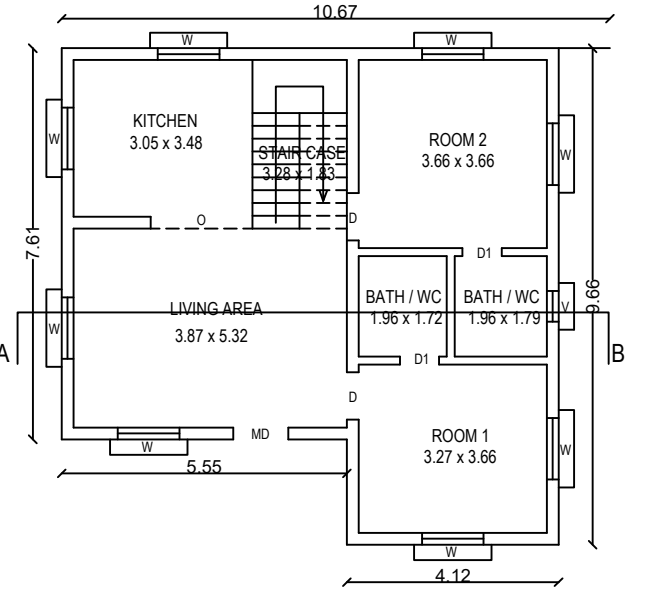
PRO GROUND FLOOR
