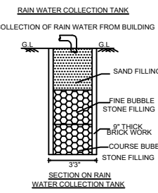
RAIN WATER COLLECTION TANK
