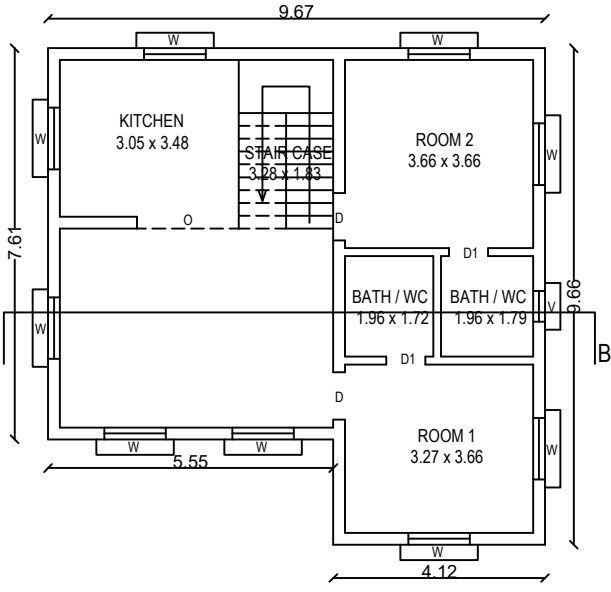
PRO FIRST FLOOR
