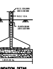
FOUNDATION DETAIL
