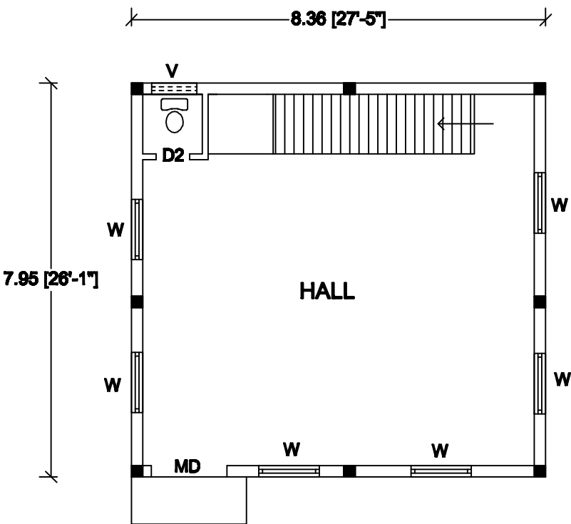
FLOOR 01
