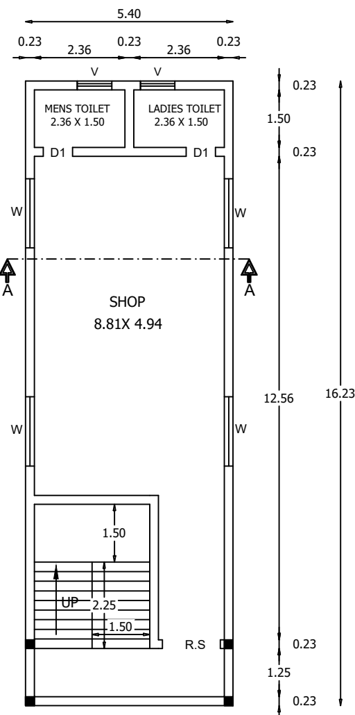
FIRST FLOOR
