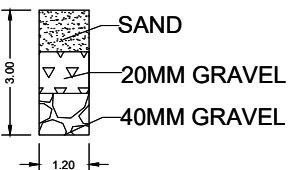
RWH DETAILS
