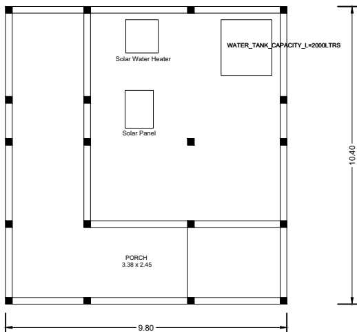
TERRACE FLOOR
