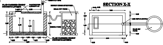
DETAIL OF SEPTIC TANK [ SCALE 1:200 ]
