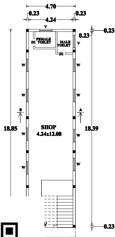
GROUND FLOOR PLAN (Commercial)
