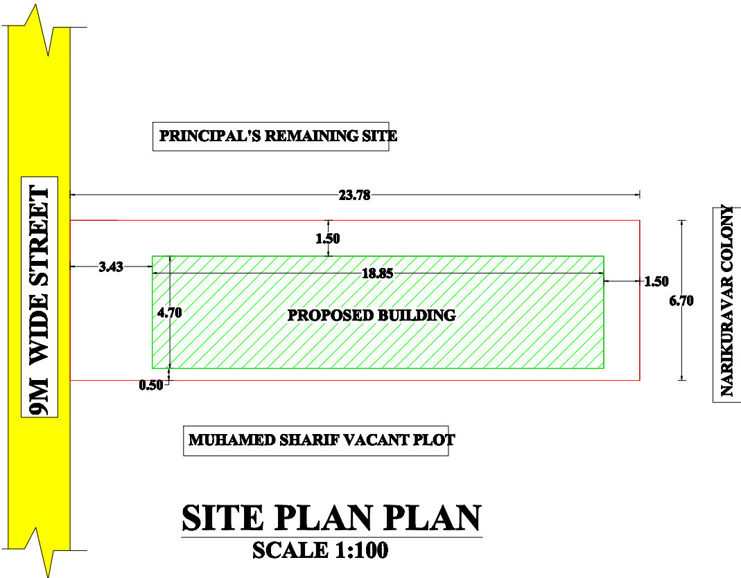
SCALE : 1:100 [ 1"= 8'0" ]
